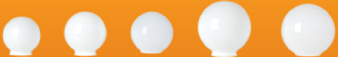
MODELO R5C/C R6C/C R6S/C R8C/C R8S/C FIGURA GLOBO C/C GLOBO C/C GLOBO S/C GLOBO C/C GLOBO S/C DIAMETRO 5" 6" 6" 8" 8" ABERTURA CUELLO 3" 3 1/4" 3 1/4" 4" 4"
